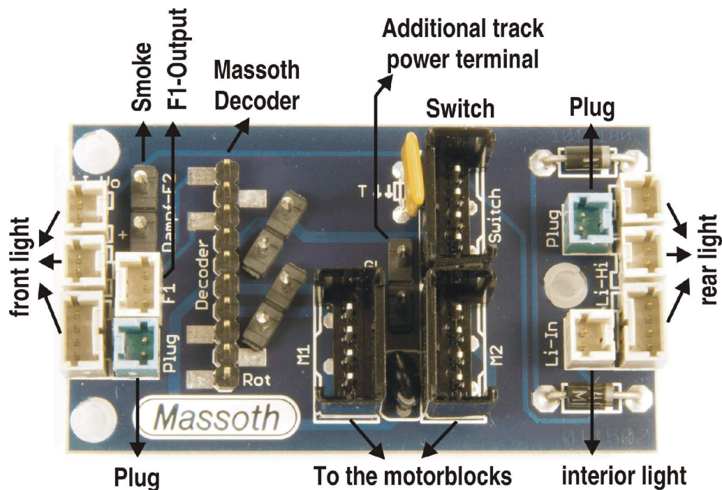
Illustration 1: Connectors of the on-board adapter
